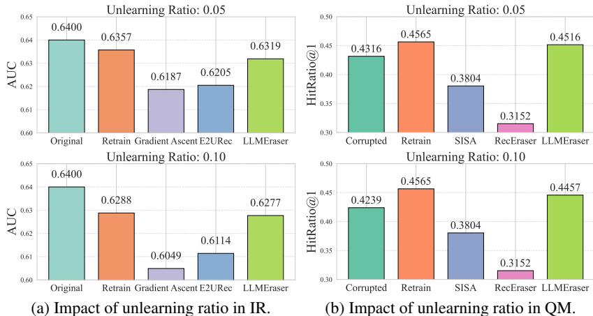
Figure 3: 3a : Experimental results of the instance removal task using TallRec as the LLM4Rec model on the BookCrossing dataset, where 5% and 10% of the training data were randomly deleted. 3b : Experimental results of the query modification task using LLaRA as the LLM4Rec model on the MovieLens dataset, where interactions were randomly removed from 5% and 10% of users.
