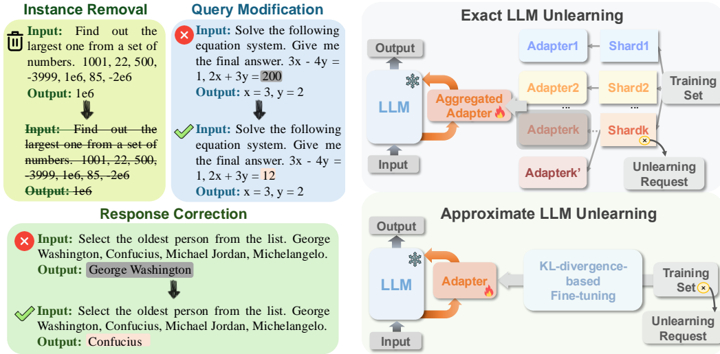
(a) Taxonomy of LLM unlearning tasks. (b) Overview of exact/approximate LLM Unlearning.
