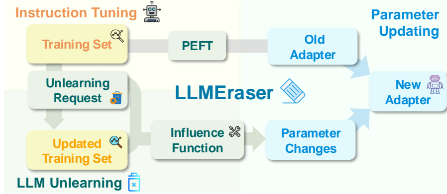
Figure 2: The framework of LLMEraser. The old adapter is obtained through PEFT on domain-specific data. When an unlearning request arrives ( e.g. , deleting or correcting certain data from the training set), LLMEraser utilizes influence functions to compute the parameter changes caused by such request. These estimated parameter modifications are added to the old adapter’s weights, resulting in the new adapter parameters—essentially the unlearned model parameters.
