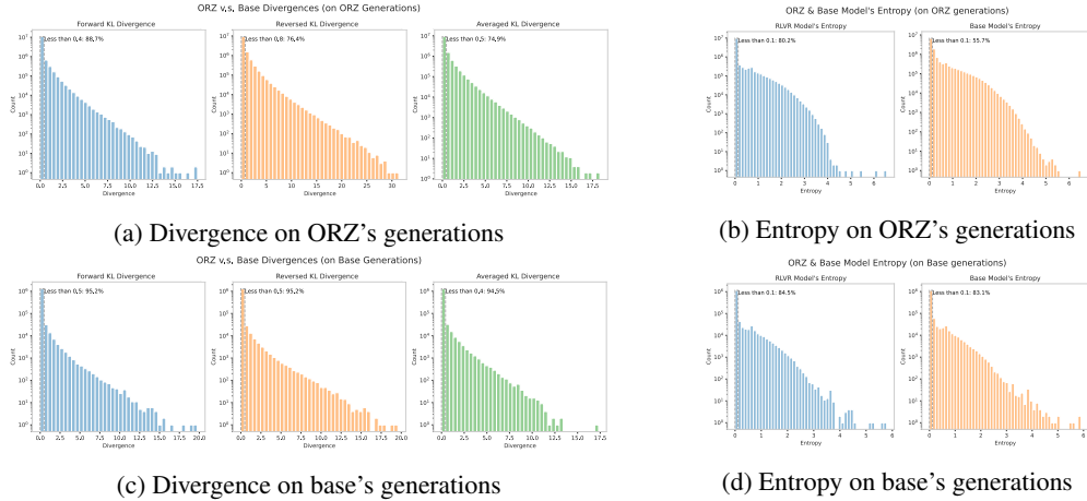
Figure 15: Divergence and entropy histograms of ORZ and its corresponding base model measured on ORZ or the base model's generations.
