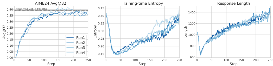
Figure 9: Reproducibility analysis. The learning curves across 4 independent runs on Qwen2.5-Math-7B with our reweighting method (Eq. 8) show consistent convergence and performance.
