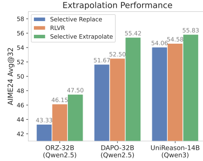
Figure 4: Extrapolation Performance
