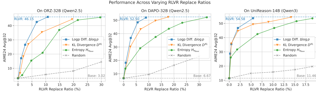
Figure 2: Token-replacement performance across metrics and model pairs. While all metrics can recover RLVLR-level accuracy, \Delta \log p does so with the fewest replacements , demonstrating its precision in isolating the reasoning-critical minor tokens changed by RLVLR training.
