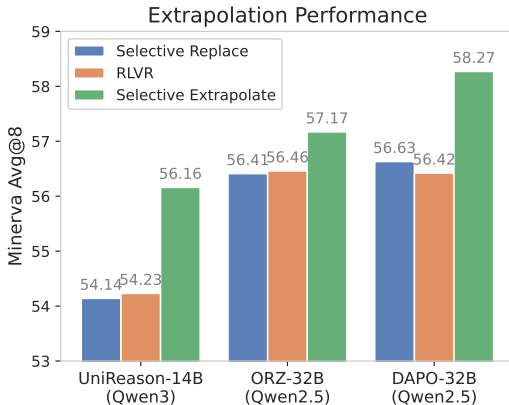
Figure 10: Extrapolation results on Minerva.
